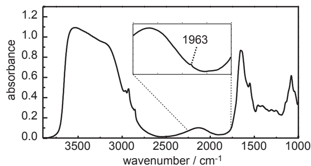
FIGURE 2 Midinfrared absorption spectrum of an aqueous solution of fully reduced, CO-bound bovine cytochrome c oxidase. The band feature between 1700 and 1500 cm -1 is associated with the amide I and II vibrations of the protein overlapped by the bending vibration of water. The high water content of the sample leads to a strong absorption \sim 3300 cm -1 (O—H stretch of water) leading to a distorted spectral shape. The bands in the region \sim 2900 cm -1 can be assigned to C—H stretching vibrations predominantly from the detergent. (Inset) Enlargement of the region \sim 2000 cm -1 where the wagging mode of water absorbs. The extremely small band at 1963 cm -1 on the shoulder of the wagging band represents the stretching vibration of bound carbon monoxide.
